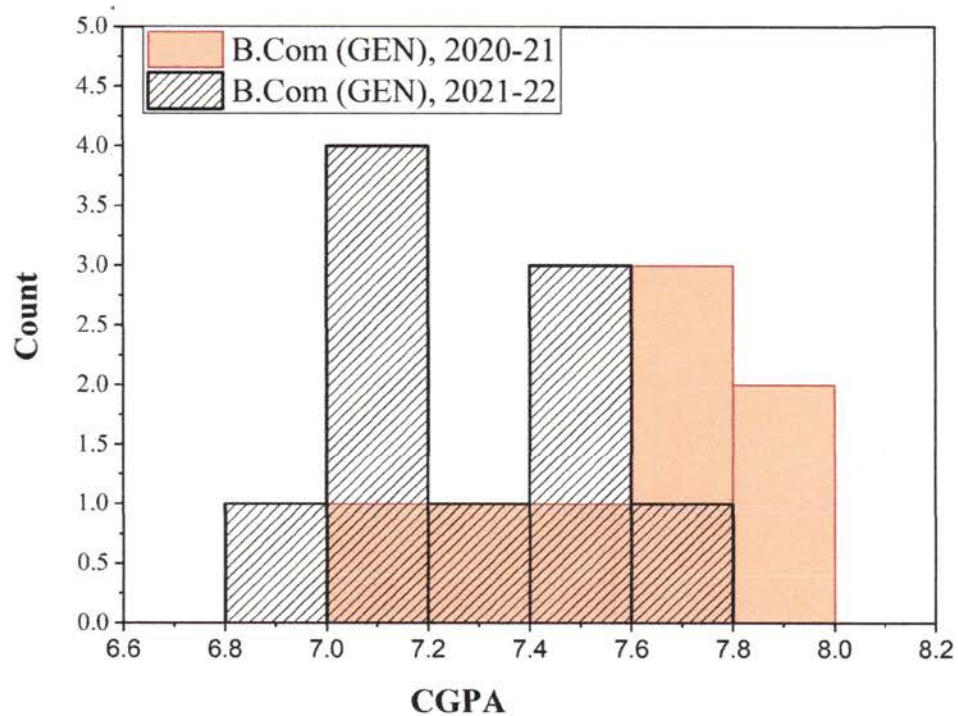
Fig.6 Distribution of grades awarded to the B.com (General) students for the academic year 2020-21 and 2021-2022.
