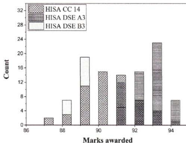
Fig.7 Distribution of marks awarded to the B.A HISA (History Honours) students for the academic year 2020-21.
