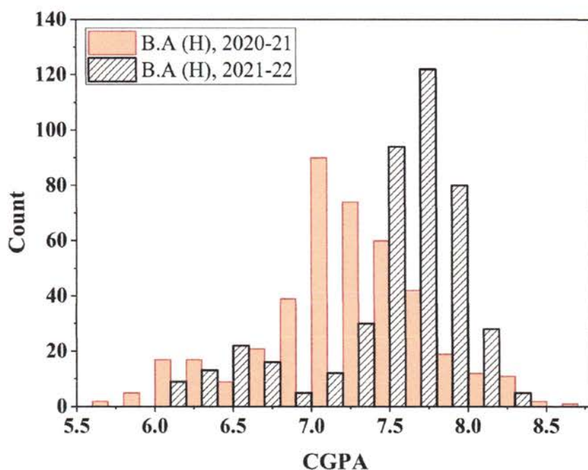
Fig. 1 Distribution of grades awarded to the B.A (Honours) students for the academic year 2020-21 and 2021-22.
