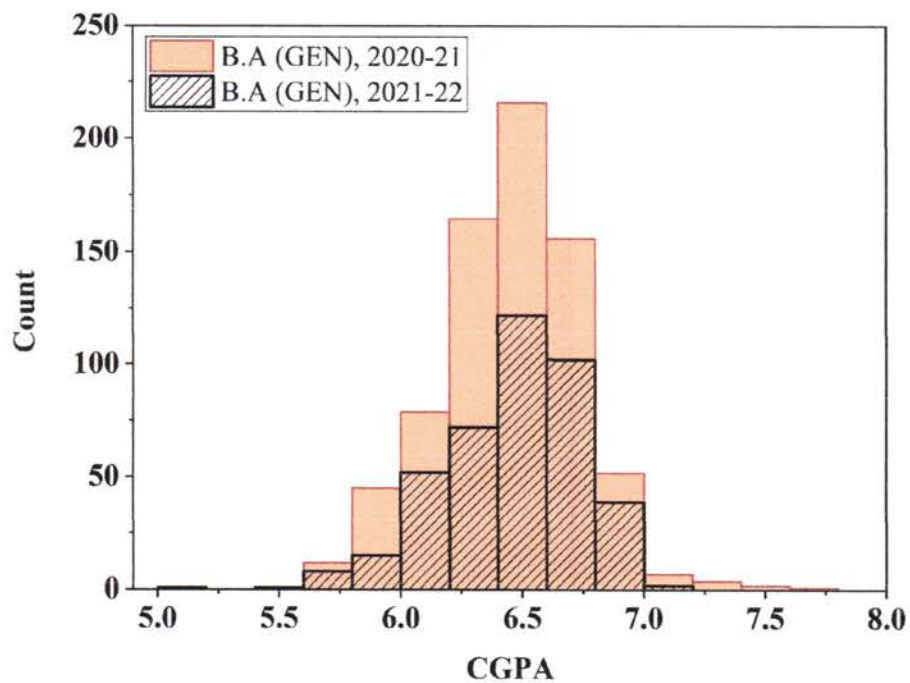
Fig.4 Distribution of grades awarded to the B.A(General) students for the academic year 2020-21 and 2021-2022.
