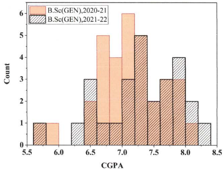
Fig.5 Distribution of grades awarded to the B.Sc (General) students for the academic year 2020-21 and 2021-2022.
