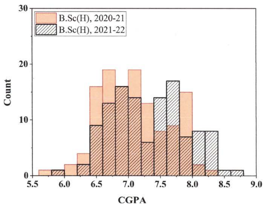
Fig. 2 Distribution of grades awarded to the B.Sc (Honours) students for the academic year 2020-21 and 2021-22.
