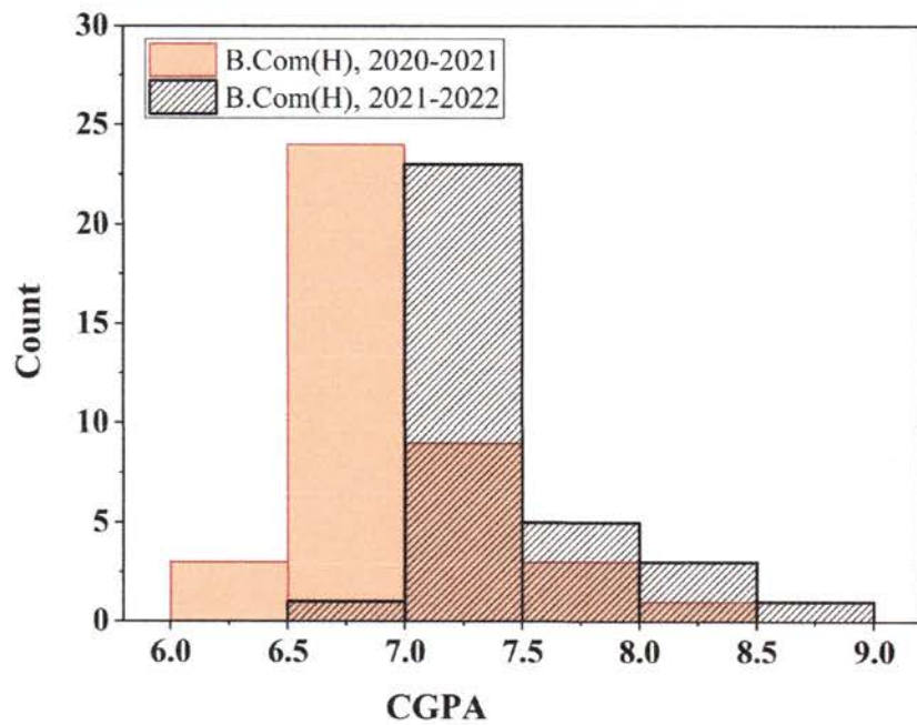
Fig.3 Distribution of grades awarded to the B.Com (Honours) students for the academic year 2020-21 and 2021-2022.
