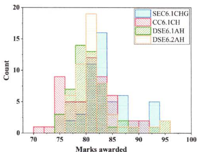
Fig.8 Distribution of marks awarded to the B.Sc PHSA (Physics Honours) students for the academic year 2020-21.
